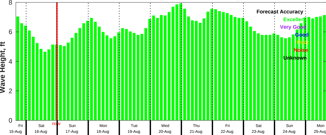
CMEMS Wave Forecast for NDBC 46028 from 15-Aug-2025 16:00:00 to 25-Aug-2025 16:00:00
