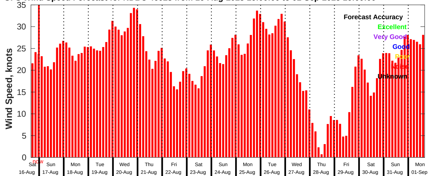
GFS Wind Speed Forecast for NDBC 46028 from 16-Aug-2025 16:00:00 to 01-Sep-2025 16:00:00
