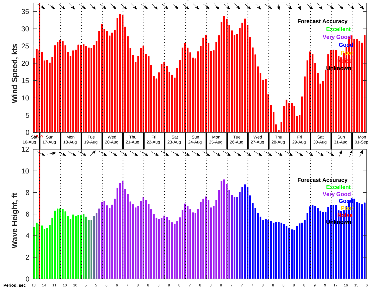
Wind & Wave Forecast for NDBC 46028 from 16-Aug-2025 16:00:00 to 01-Sep-2025 16:00:00
