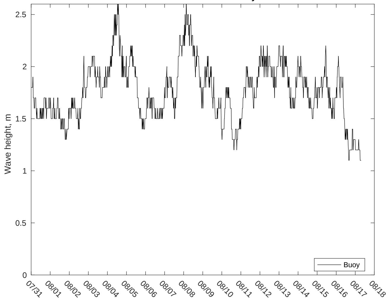
NDBC 46054 vs CMEMS Waves: 10 to 16 day forecast
