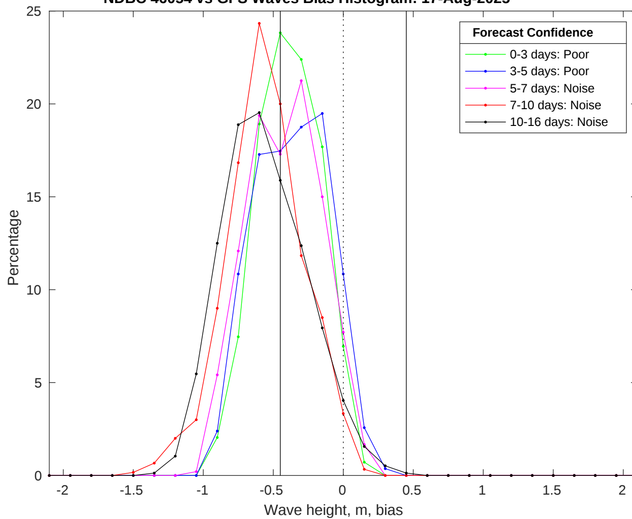
NDBC 46054 vs GFS Waves Bias Histogram: 17-Aug-2025
