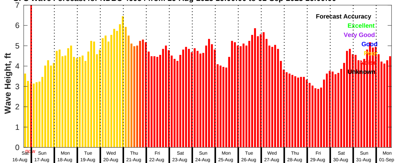
GFS Wave Forecast for NDBC 46054 from 16-Aug-2025 16:00:00 to 01-Sep-2025 16:00:00
