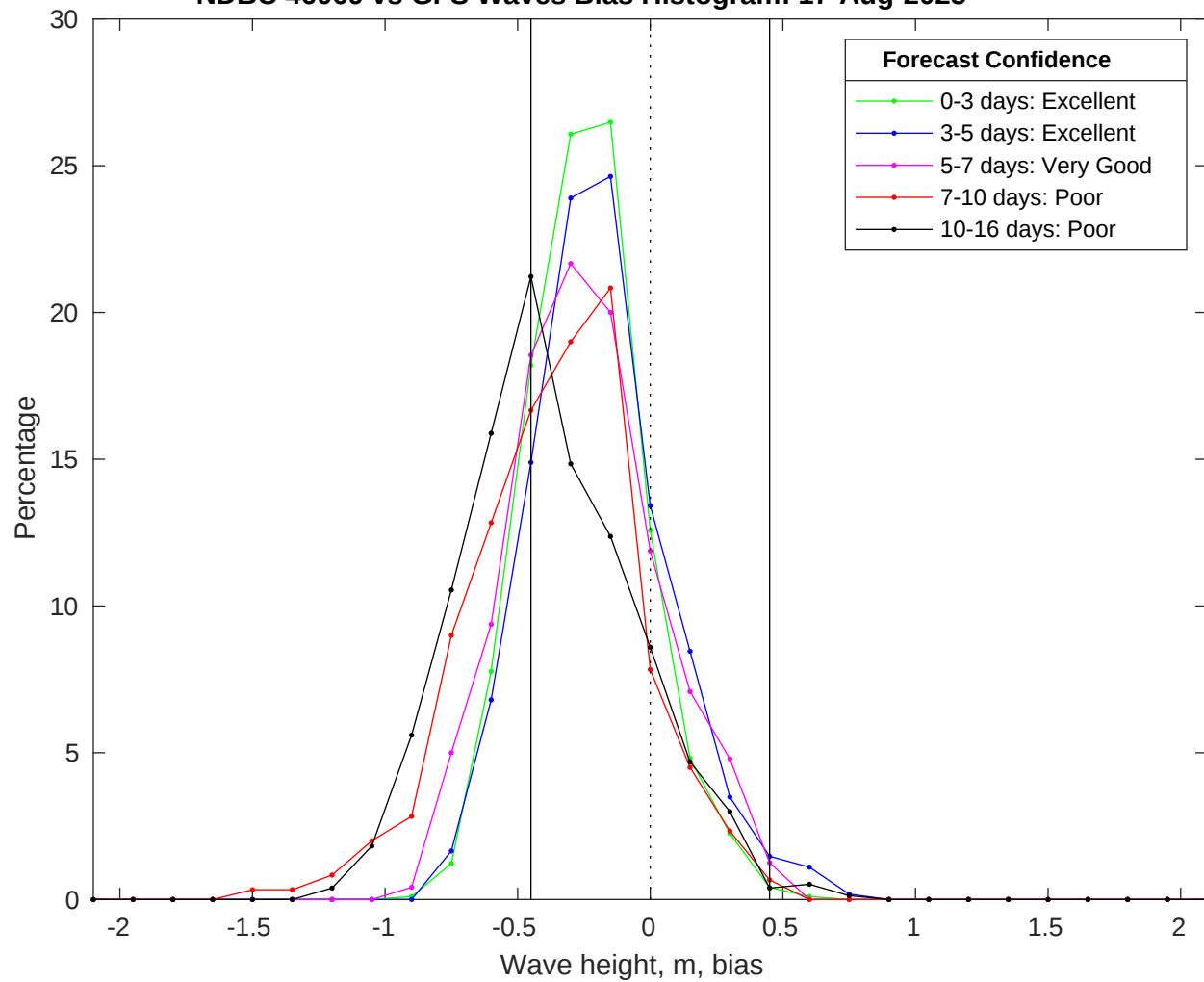
NDBC 46069 vs GFS Waves Bias Histogram: 17-Aug-2025
