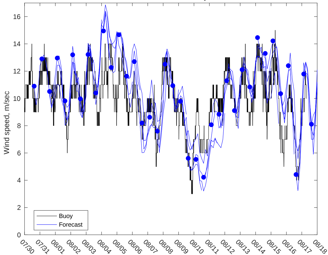
NDBC 46069 vs GFS Winds: 3 to 5 day forecast
