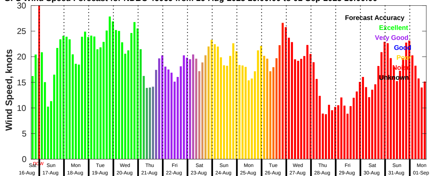
GFS Wind Speed Forecast for NDBC 46069 from 16-Aug-2025 16:00:00 to 01-Sep-2025 16:00:00
