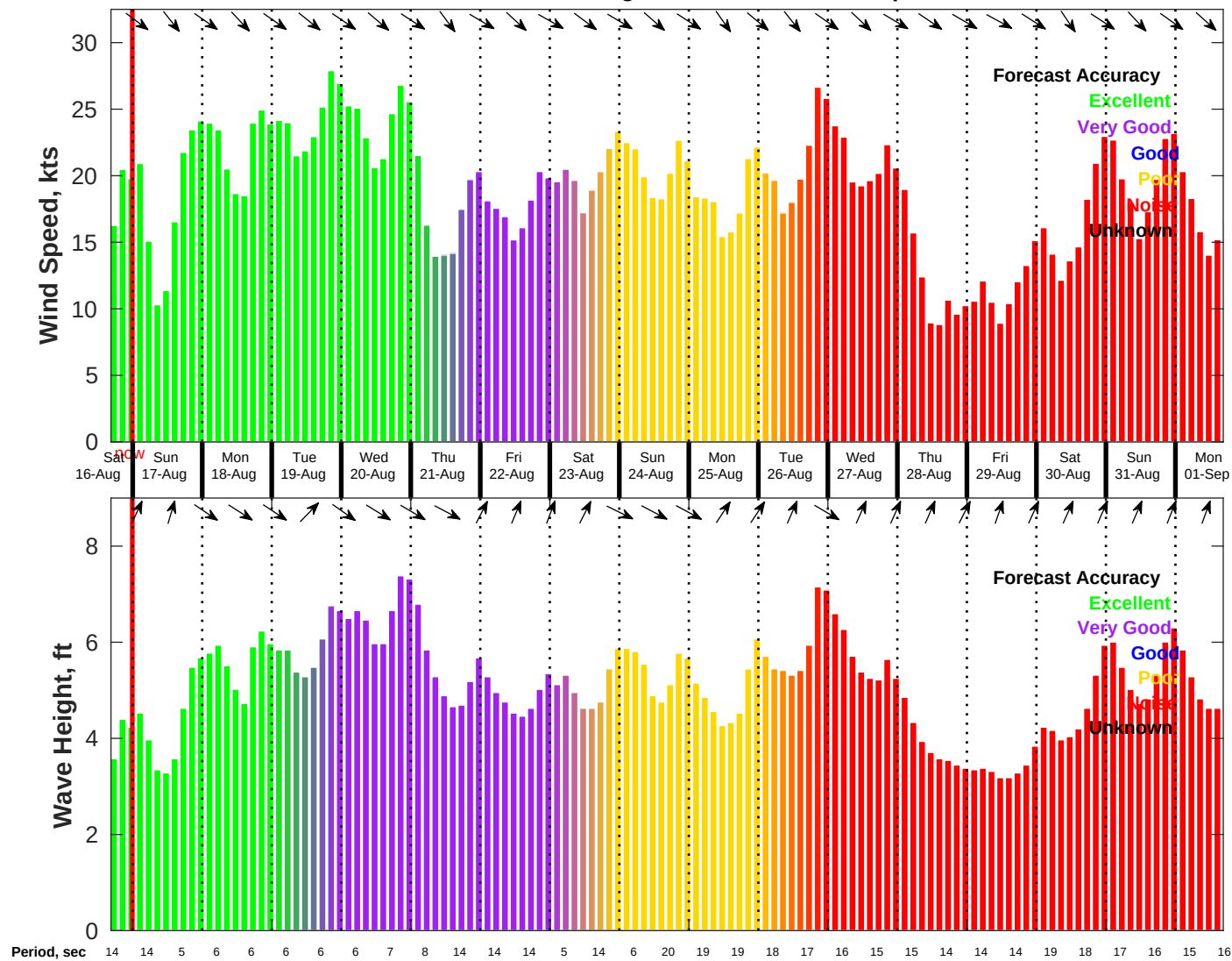
Wind & Wave Forecast for NDBC 46069 from 16-Aug-2025 16:00:00 to 01-Sep-2025 16:00:00
