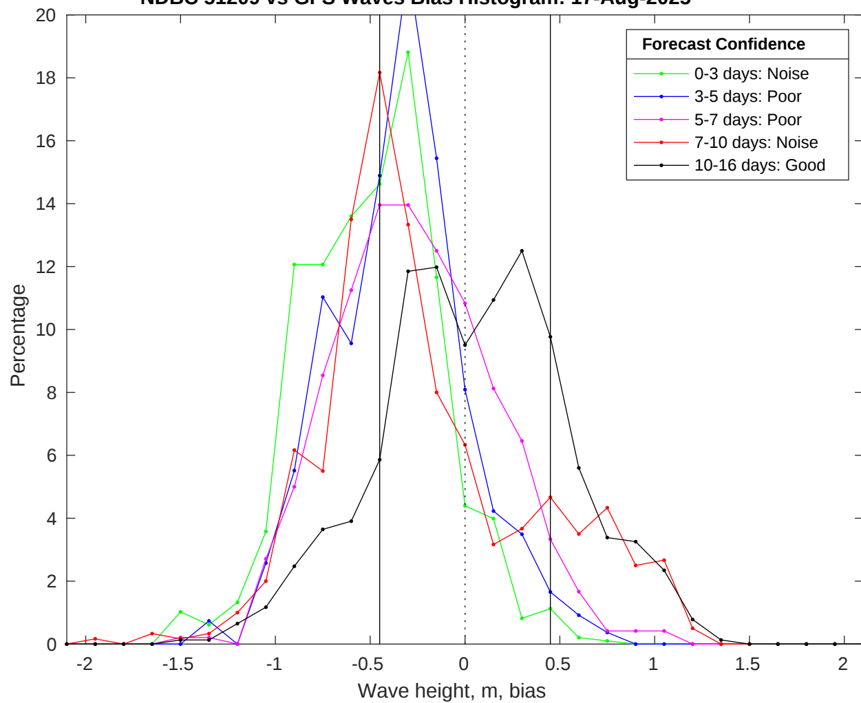
NDBC 51209 vs GFS Waves Bias Histogram: 17-Aug-2025
