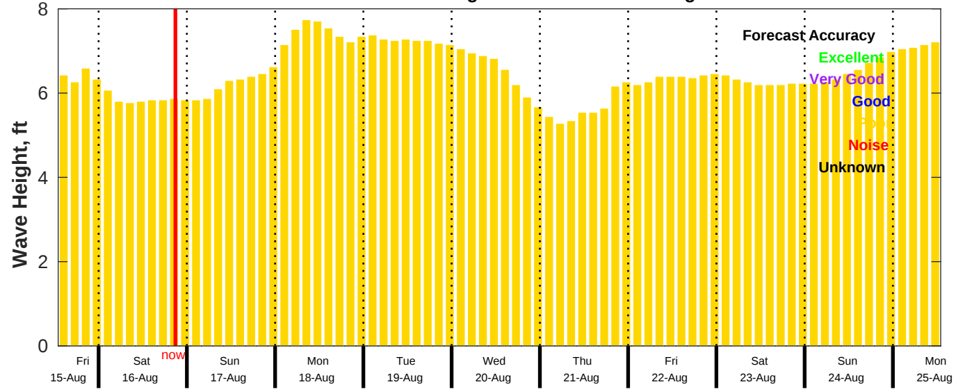
CMEMS Wave Forecast for NDBC 51209 from 15-Aug-2025 13:00:00 to 25-Aug-2025 13:00:00
