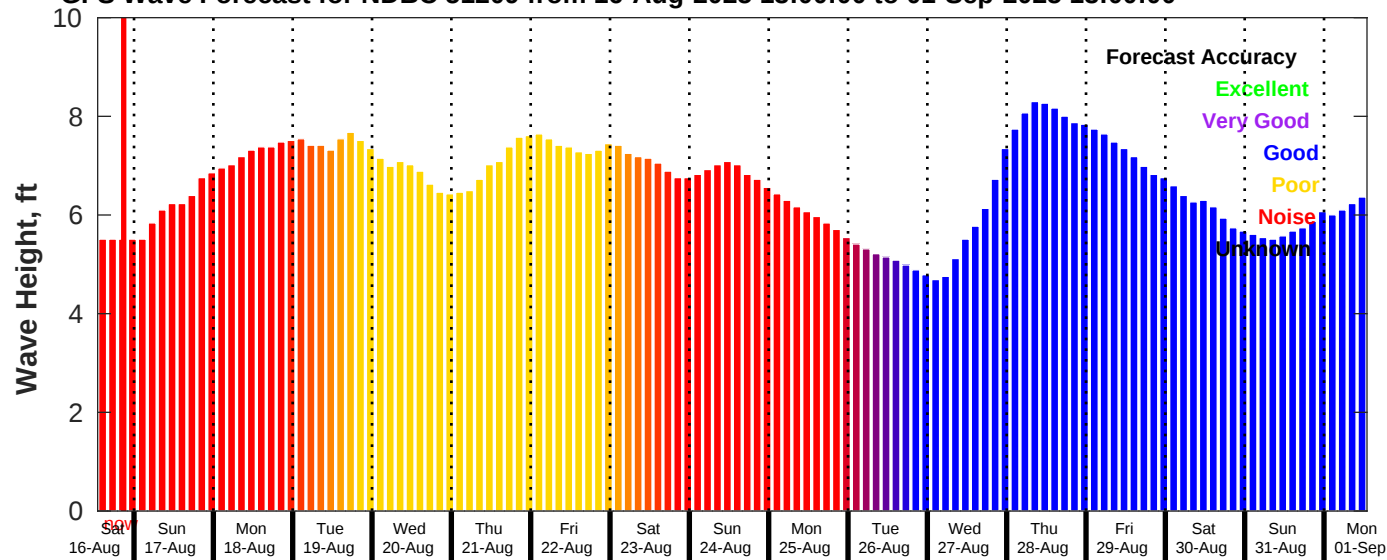
GFS Wave Forecast for NDBC 51209 from 16-Aug-2025 13:00:00 to 01-Sep-2025 13:00:00
