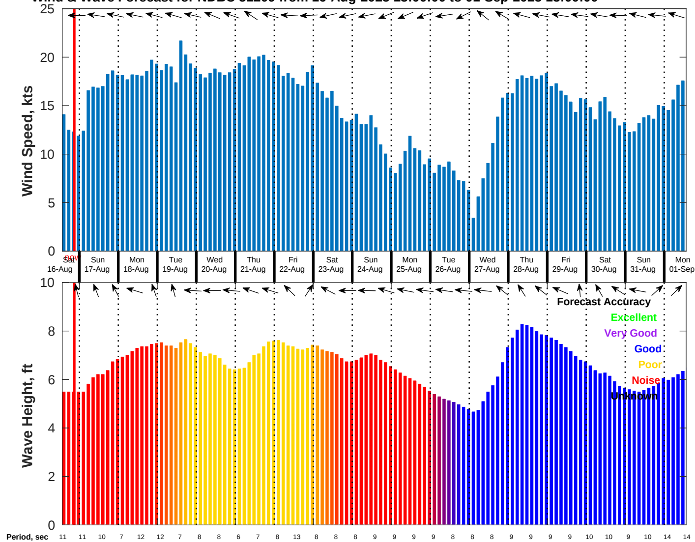
Wind & Wave Forecast for NDBC 51209 from 16-Aug-2025 13:00:00 to 01-Sep-2025 13:00:00
