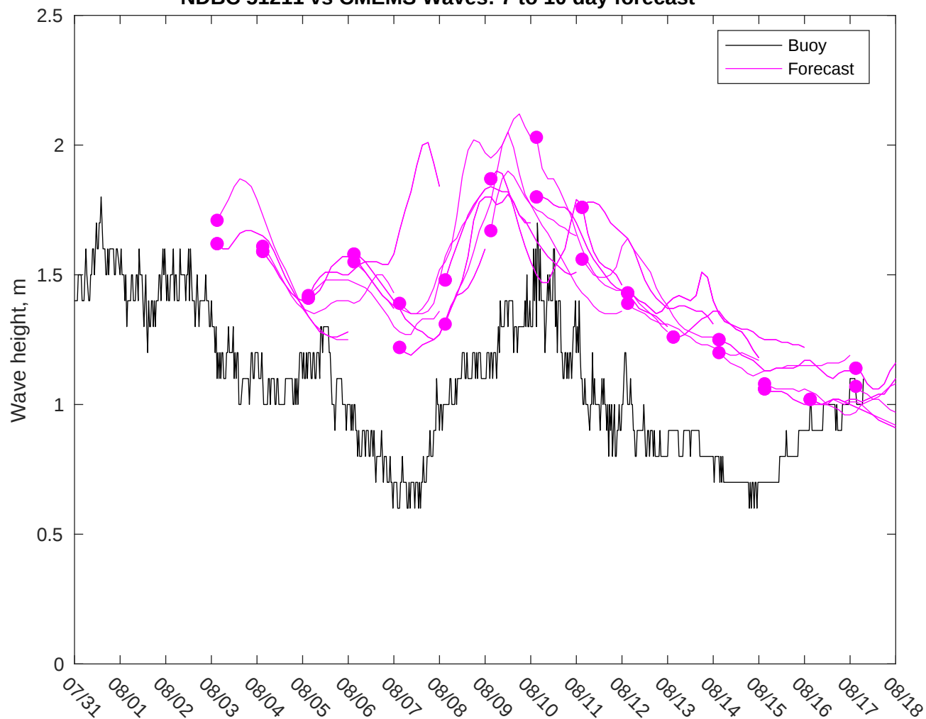
NDBC 51211 vs CMEMS Waves: 7 to 10 day forecast
