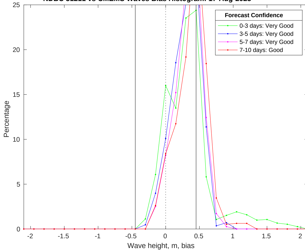
NDBC 51211 vs CMEMS Waves Bias Histogram: 17-Aug-2025
