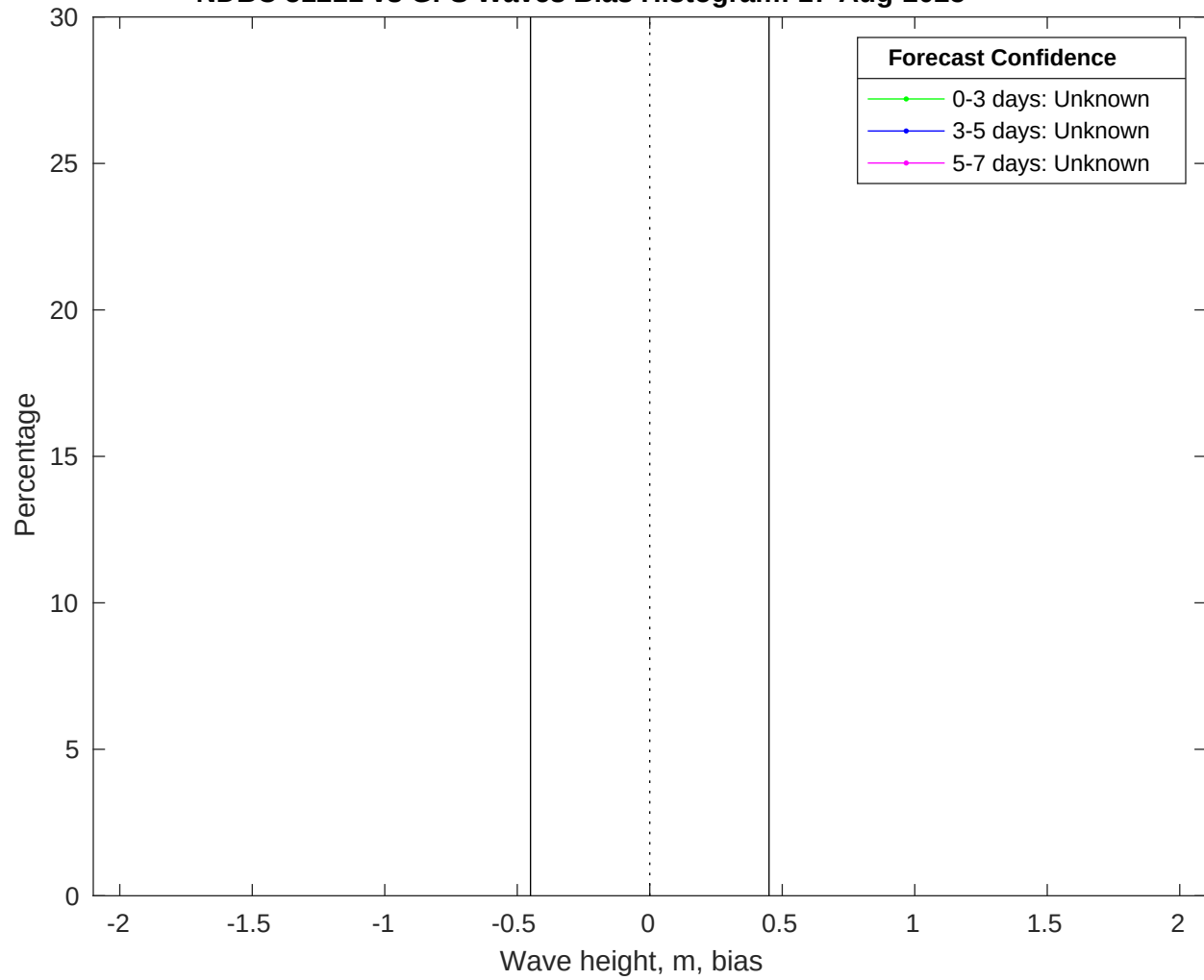
NDBC 51211 vs GFS Waves Bias Histogram: 17-Aug-2025
