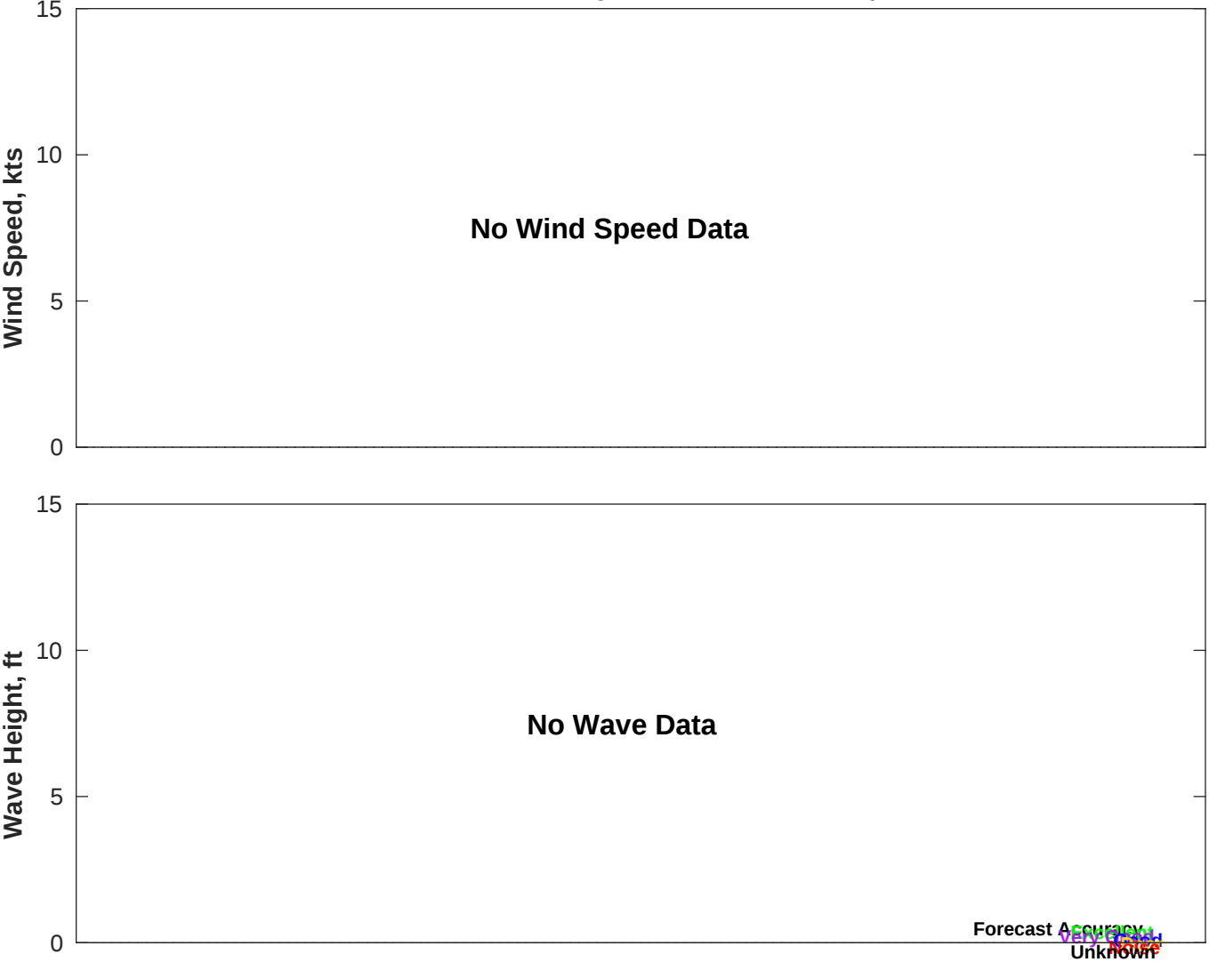
Wind & Wave Forecast for NDBC 51211 from 16-Aug-2025 14:00:00 to 01-Sep-2025 14:00:00
