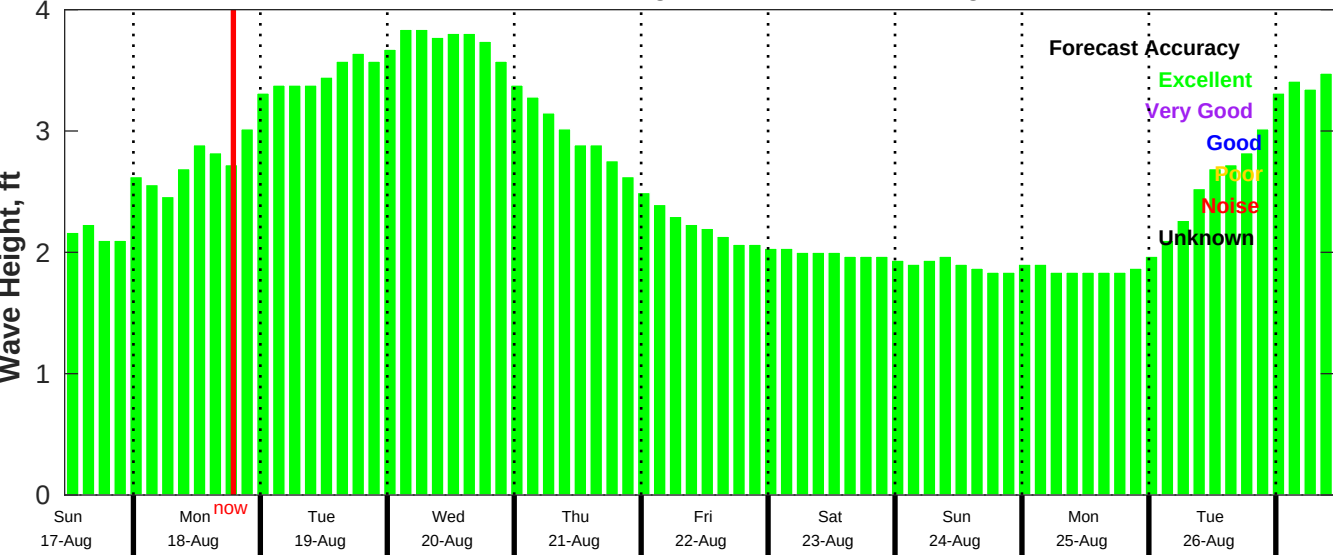
CMEMS Wave Forecast for NDBC 52211 from 16-Aug-2025 11:00:00 to 26-Aug-2025 11:00:00
