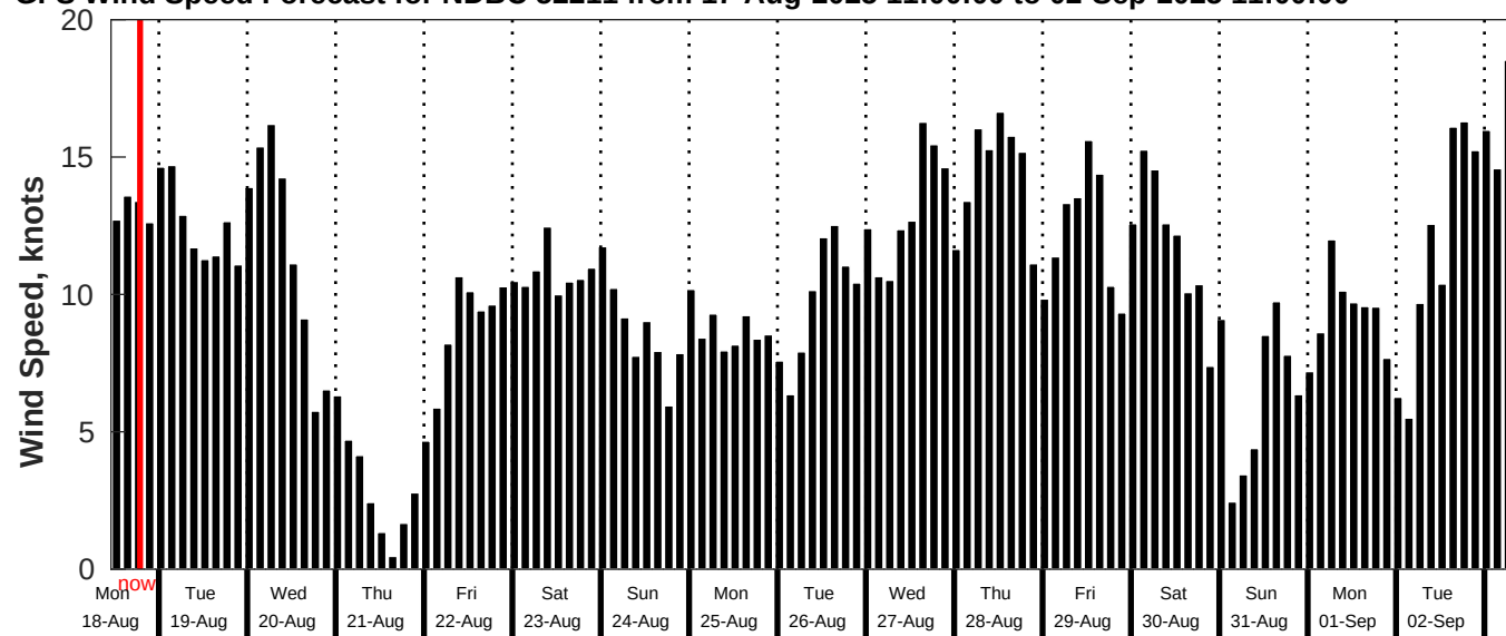
GFS Wind Speed Forecast for NDBC 52211 from 17-Aug-2025 11:00:00 to 02-Sep-2025 11:00:00
