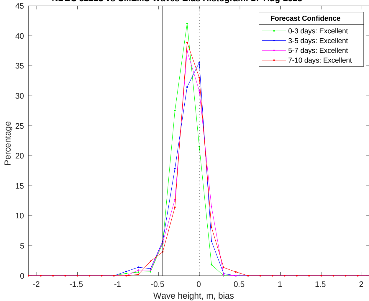
NDBC 52213 vs CMEMS Waves Bias Histogram: 17-Aug-2025
