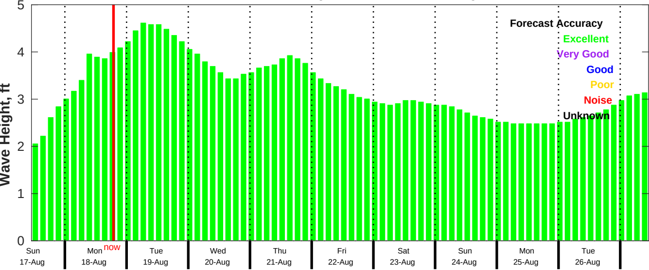
CMEMS Wave Forecast for NDBC 52213 from 16-Aug-2025 11:00:00 to 26-Aug-2025 11:00:00
