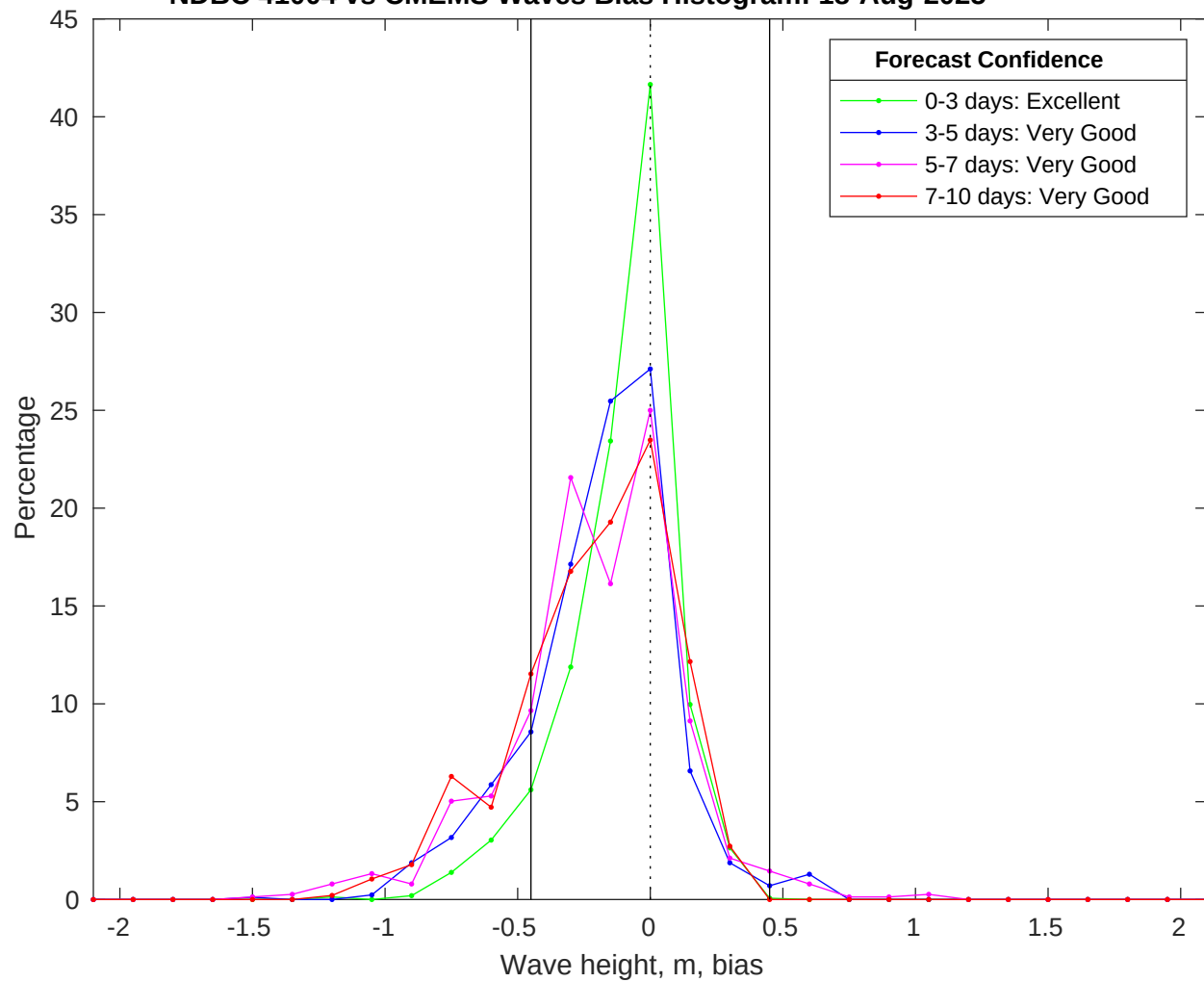
NDBC 41004 vs CMEMS Waves Bias Histogram: 18-Aug-2025
