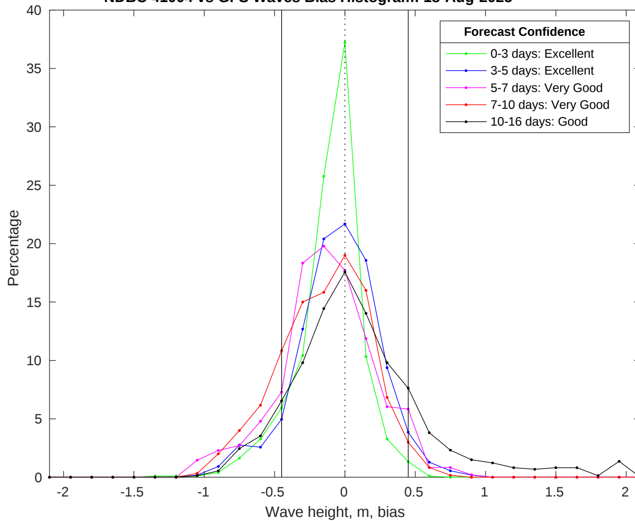
NDBC 41004 vs GFS Waves Bias Histogram: 18-Aug-2025
