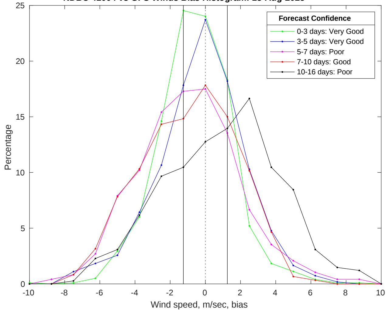
NDBC 41004 vs GFS Winds Bias Histogram: 18-Aug-2025
