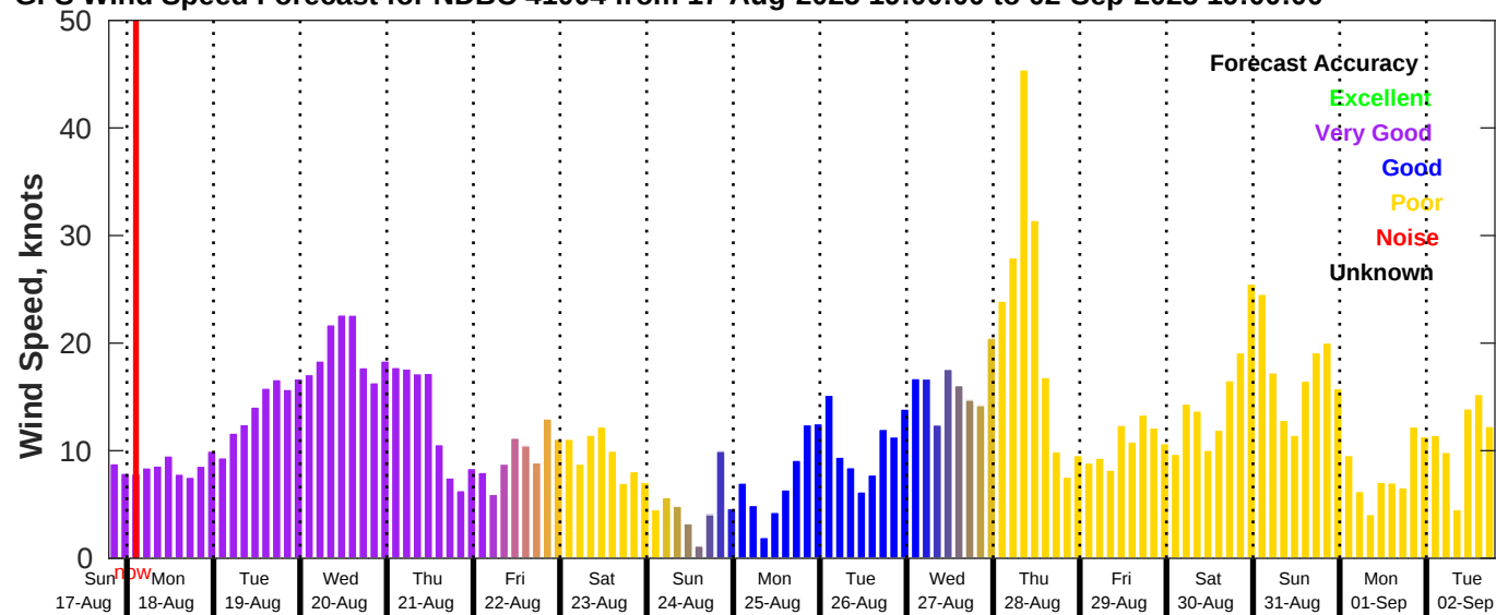
GFS Wind Speed Forecast for NDBC 41004 from 17-Aug-2025 19:00:00 to 02-Sep-2025 19:00:00
