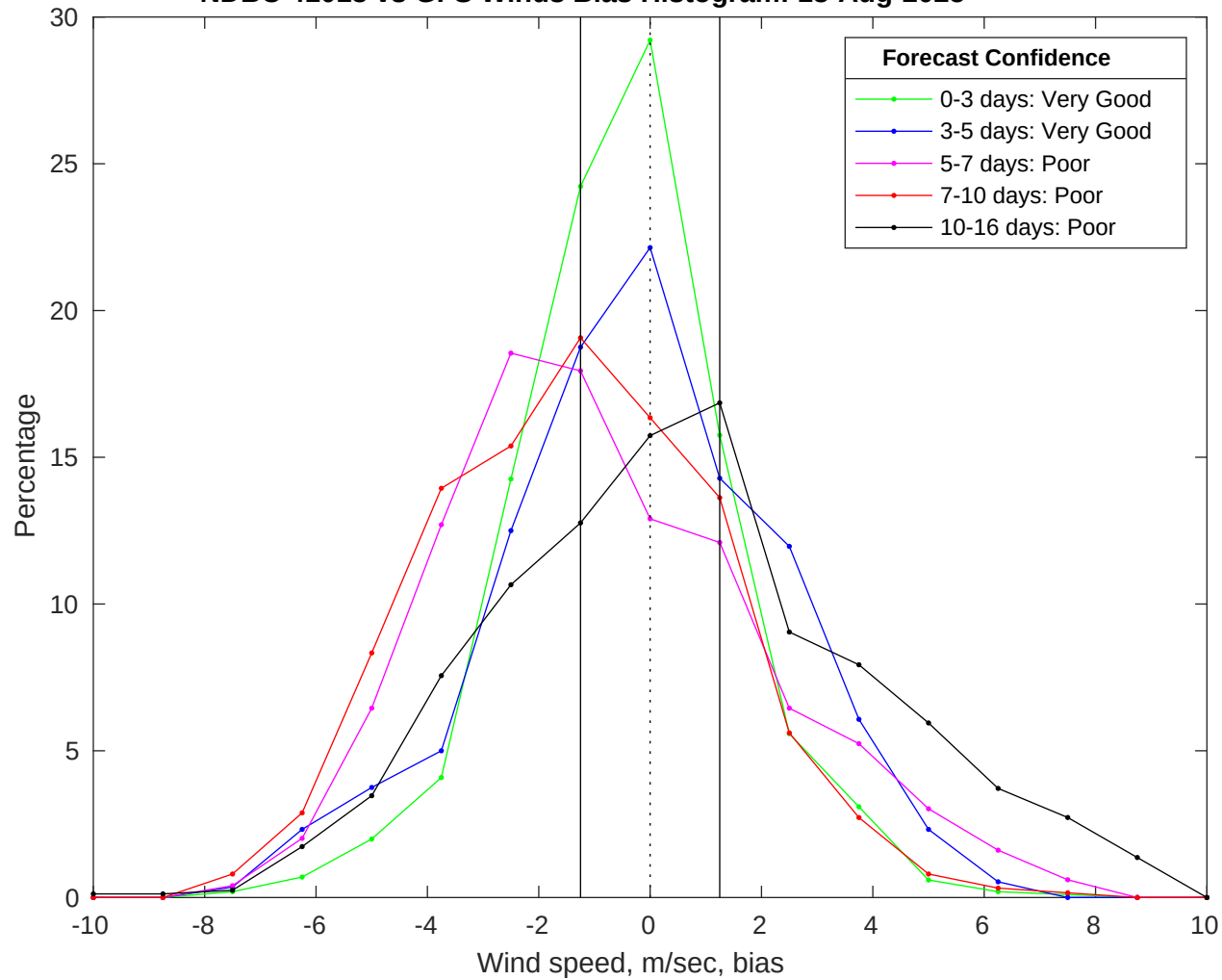
NDBC 41013 vs GFS Winds Bias Histogram: 18-Aug-2025
