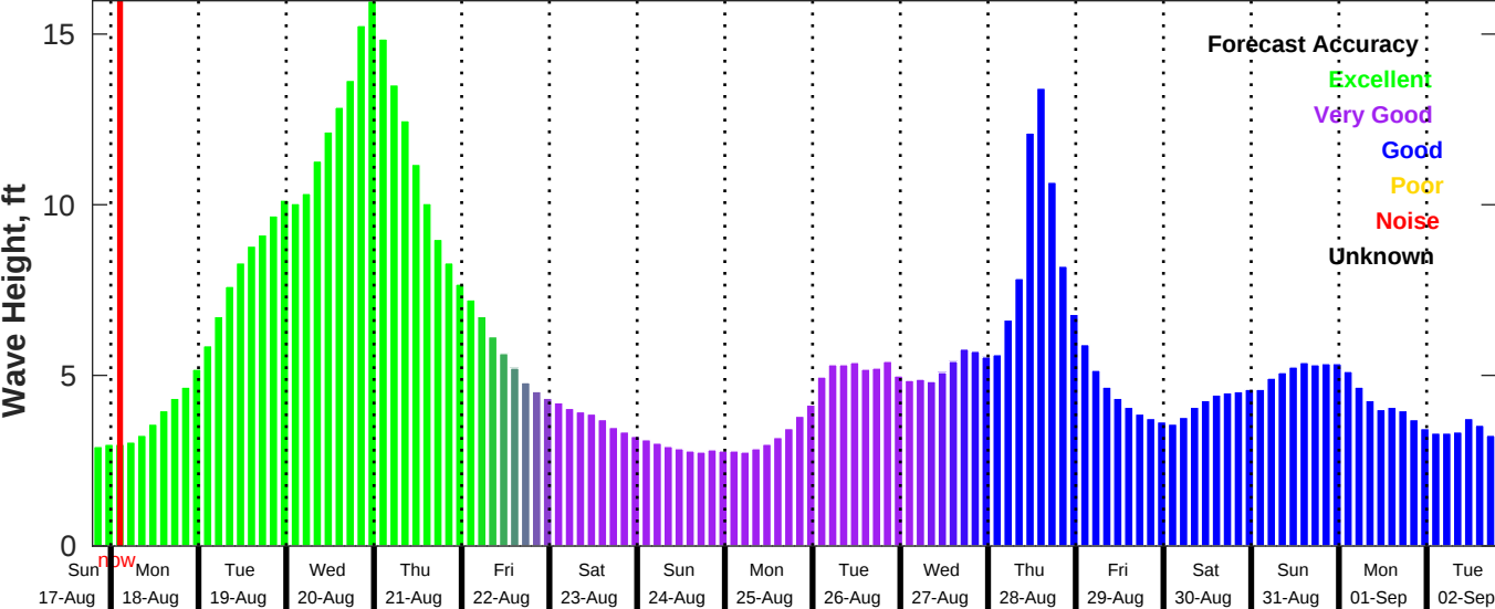
GFS Wave Forecast for NDBC 41013 from 17-Aug-2025 19:00:00 to 02-Sep-2025 19:00:00
