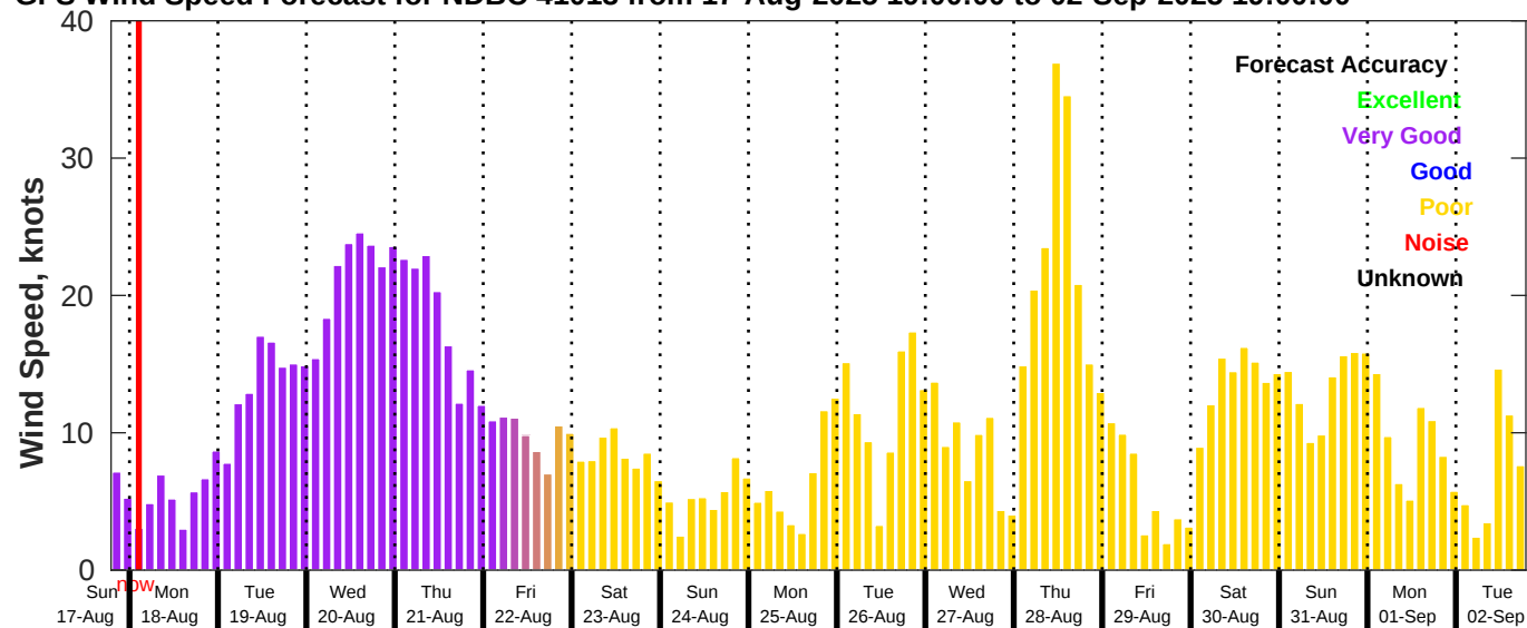
GFS Wind Speed Forecast for NDBC 41013 from 17-Aug-2025 19:00:00 to 02-Sep-2025 19:00:00
