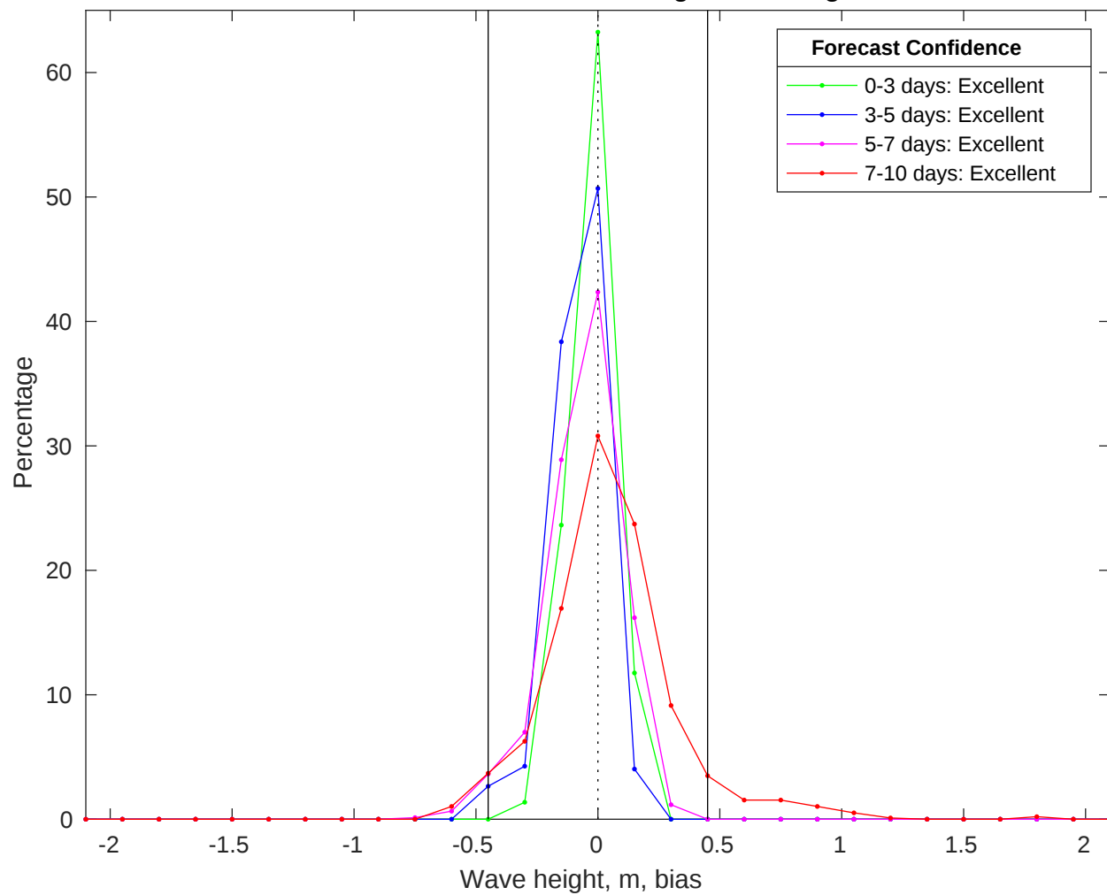
NDBC 41040 vs CMEMS Waves Bias Histogram: 18-Aug-2025
