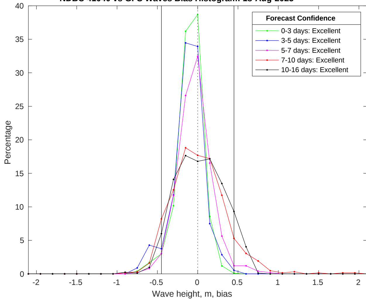
NDBC 41040 vs GFS Waves Bias Histogram: 18-Aug-2025
