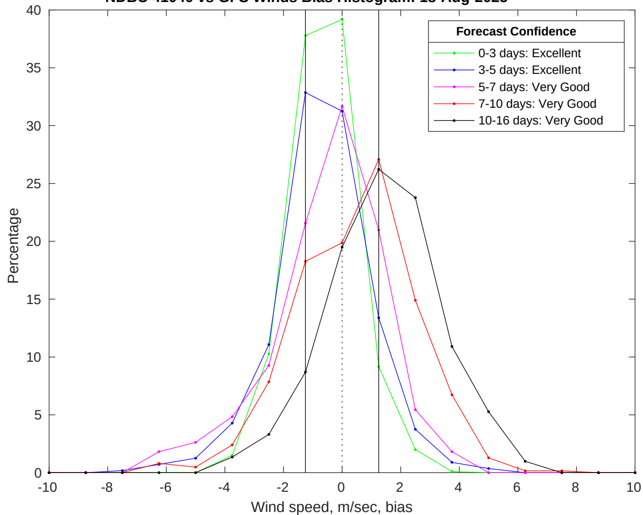
NDBC 41040 vs GFS Winds Bias Histogram: 18-Aug-2025
