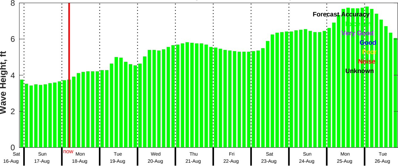
CMEMS Wave Forecast for NDBC 41040 from 16-Aug-2025 21:00:00 to 26-Aug-2025 21:00:00
