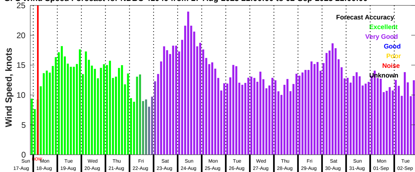
GFS Wind Speed Forecast for NDBC 41040 from 17-Aug-2025 21:00:00 to 02-Sep-2025 21:00:00
