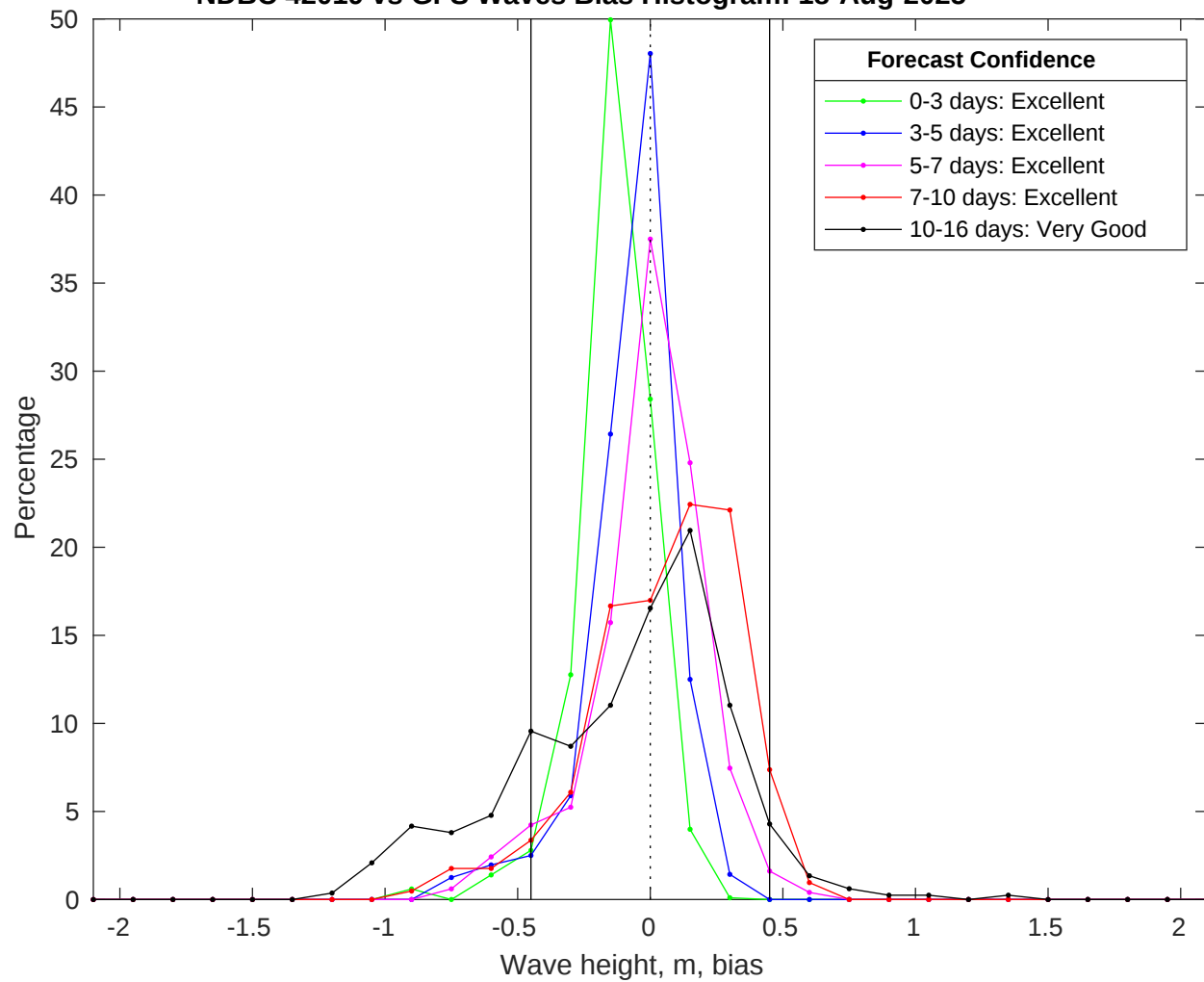
NDBC 42019 vs GFS Waves Bias Histogram: 18-Aug-2025
