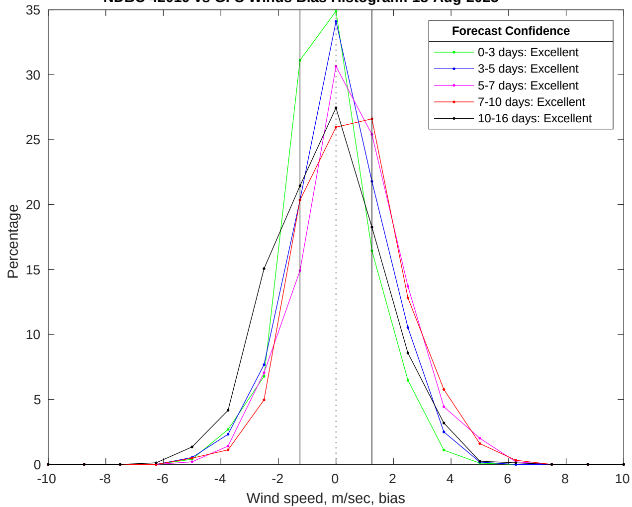
NDBC 42019 vs GFS Winds Bias Histogram: 18-Aug-2025
