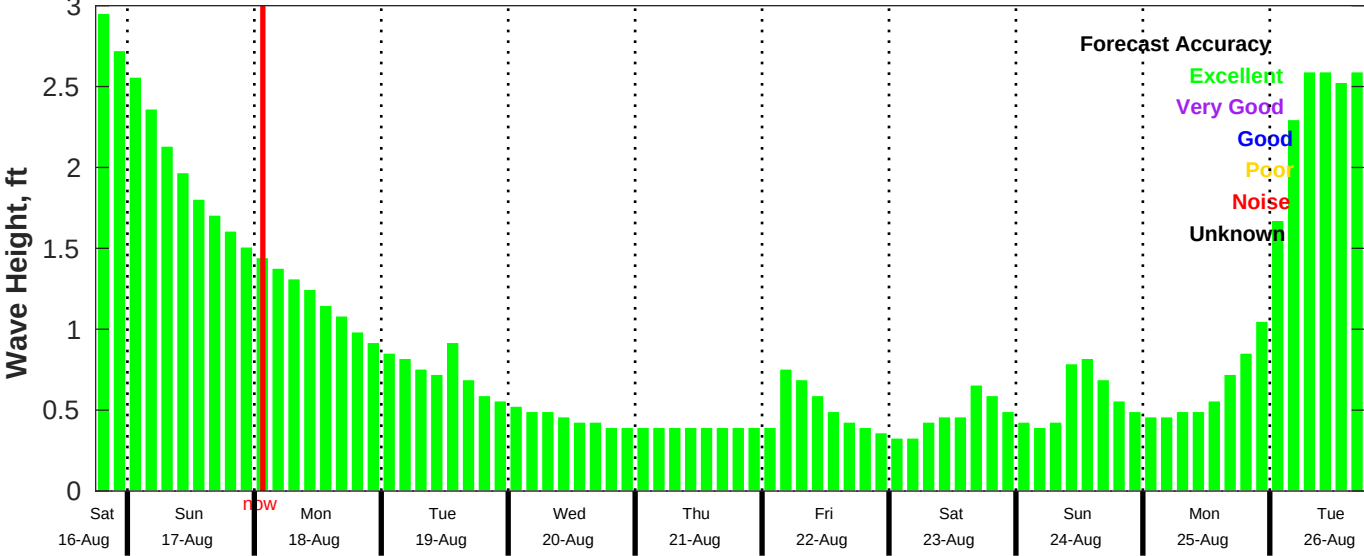
CMEMS Wave Forecast for NDBC 42019 from 16-Aug-2025 18:00:00 to 26-Aug-2025 18:00:00
