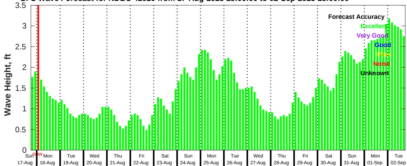
GFS Wave Forecast for NDBC 42020 from 17-Aug-2025 18:00:00 to 02-Sep-2025 18:00:00
