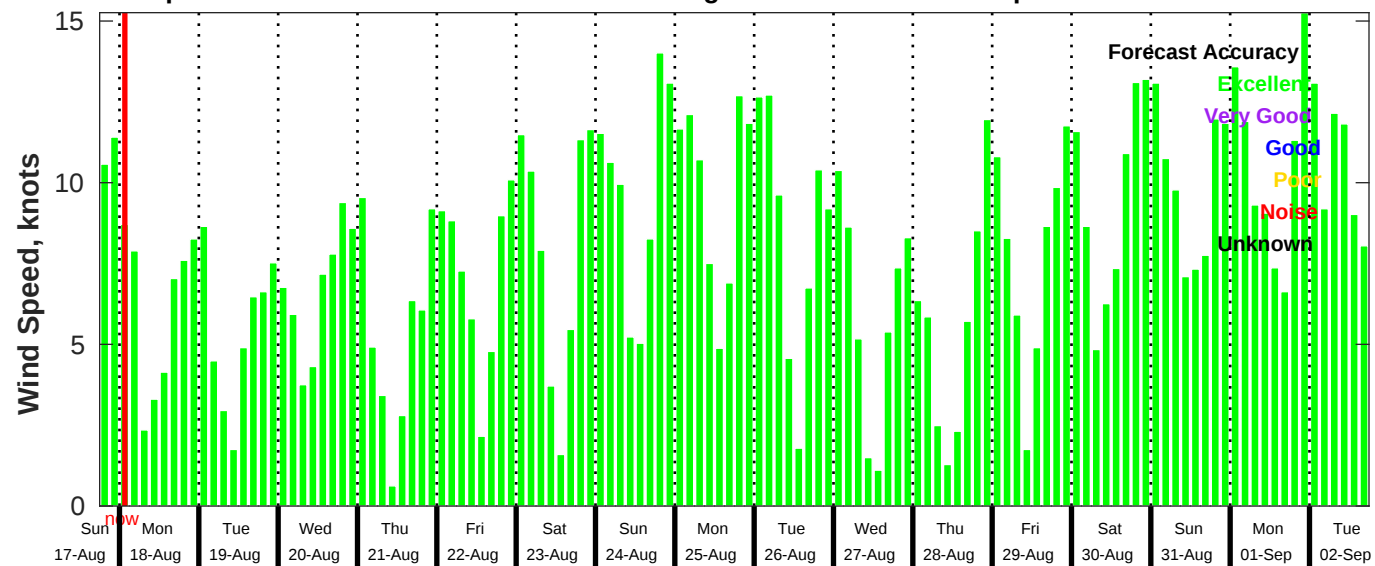
GFS Wind Speed Forecast for NDBC 42020 from 17-Aug-2025 18:00:00 to 02-Sep-2025 18:00:00
