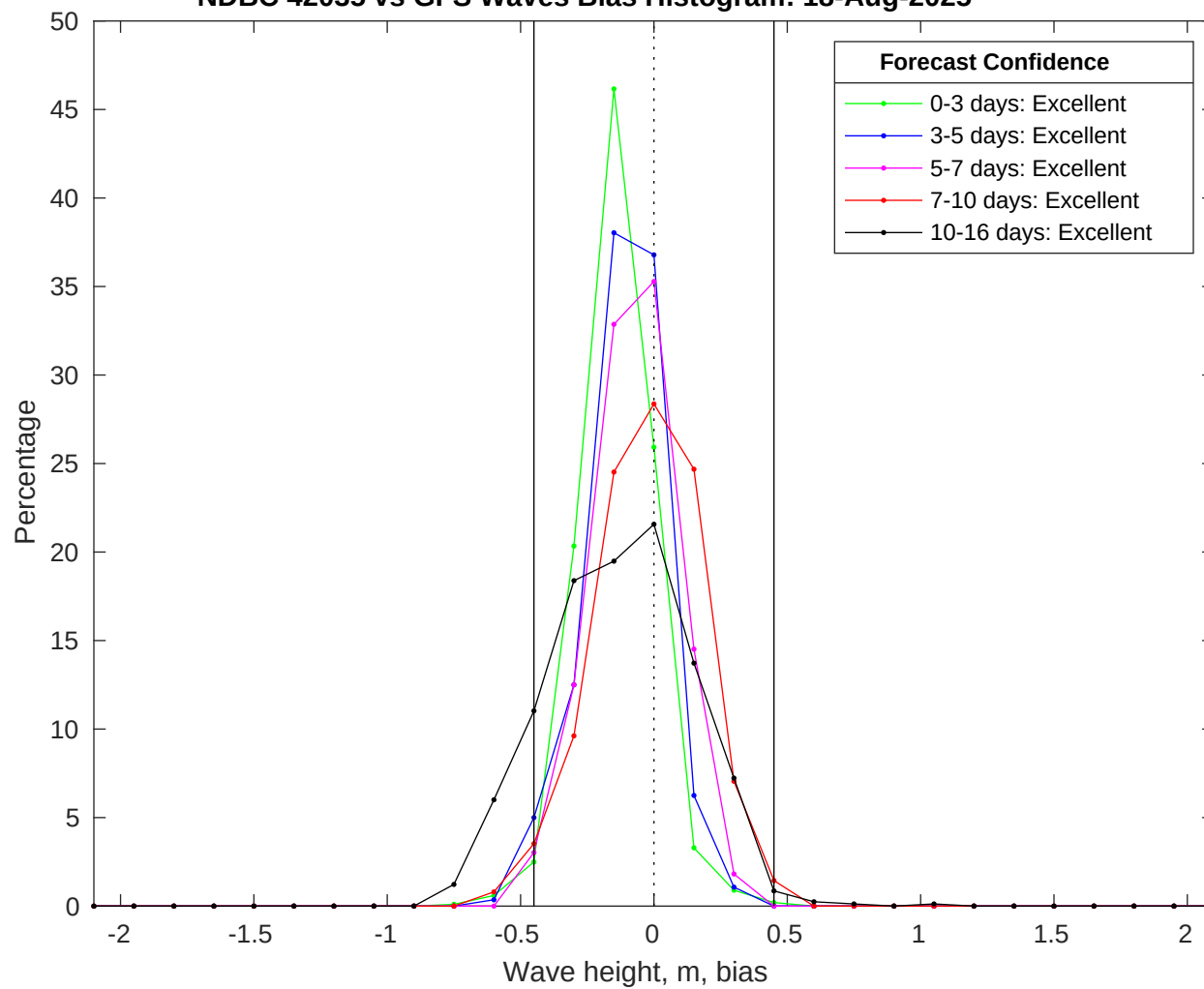
NDBC 42035 vs GFS Waves Bias Histogram: 18-Aug-2025
