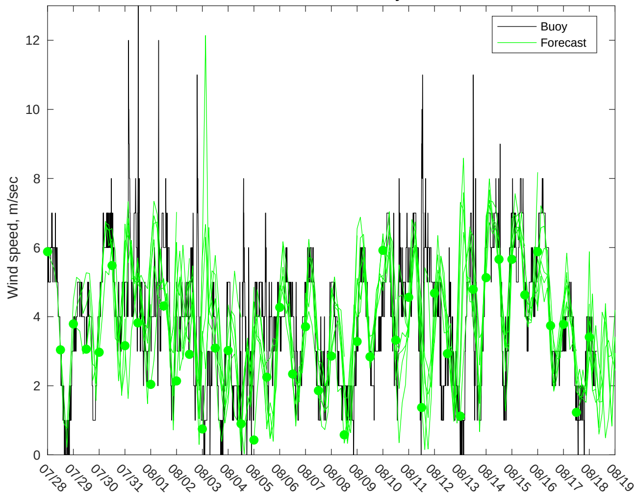
NDBC 42035 vs GFS Winds: 0 to 3 day forecast
