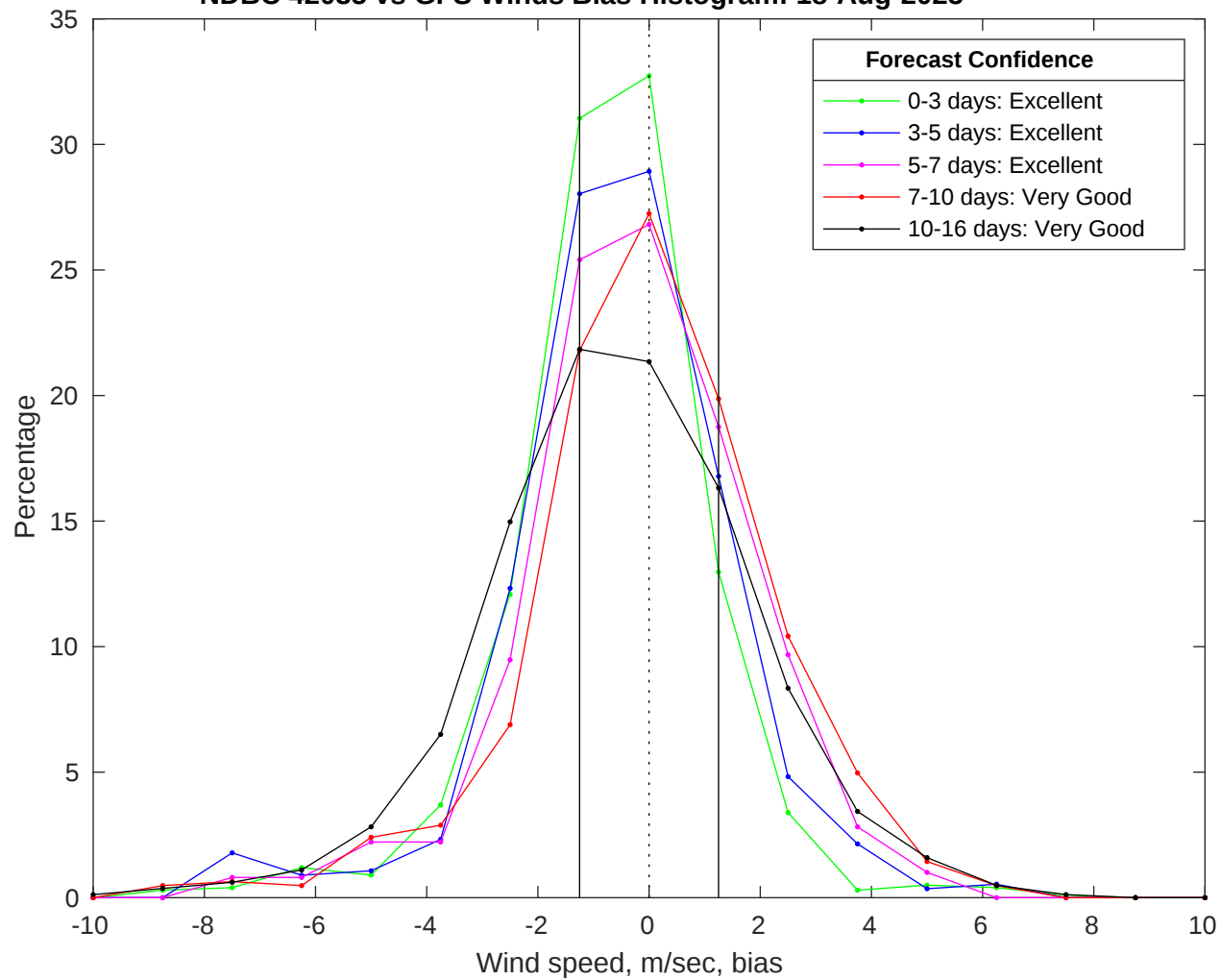
NDBC 42035 vs GFS Winds Bias Histogram: 18-Aug-2025
