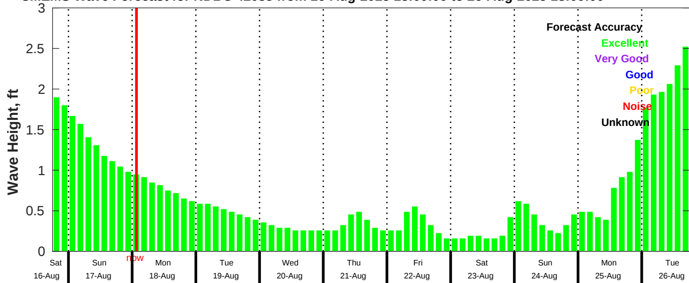
CMEMS Wave Forecast for NDBC 42035 from 16-Aug-2025 18:00:00 to 26-Aug-2025 18:00:00
