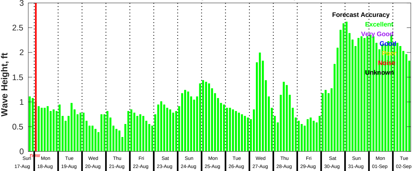
GFS Wave Forecast for NDBC 42035 from 17-Aug-2025 18:00:00 to 02-Sep-2025 18:00:00
