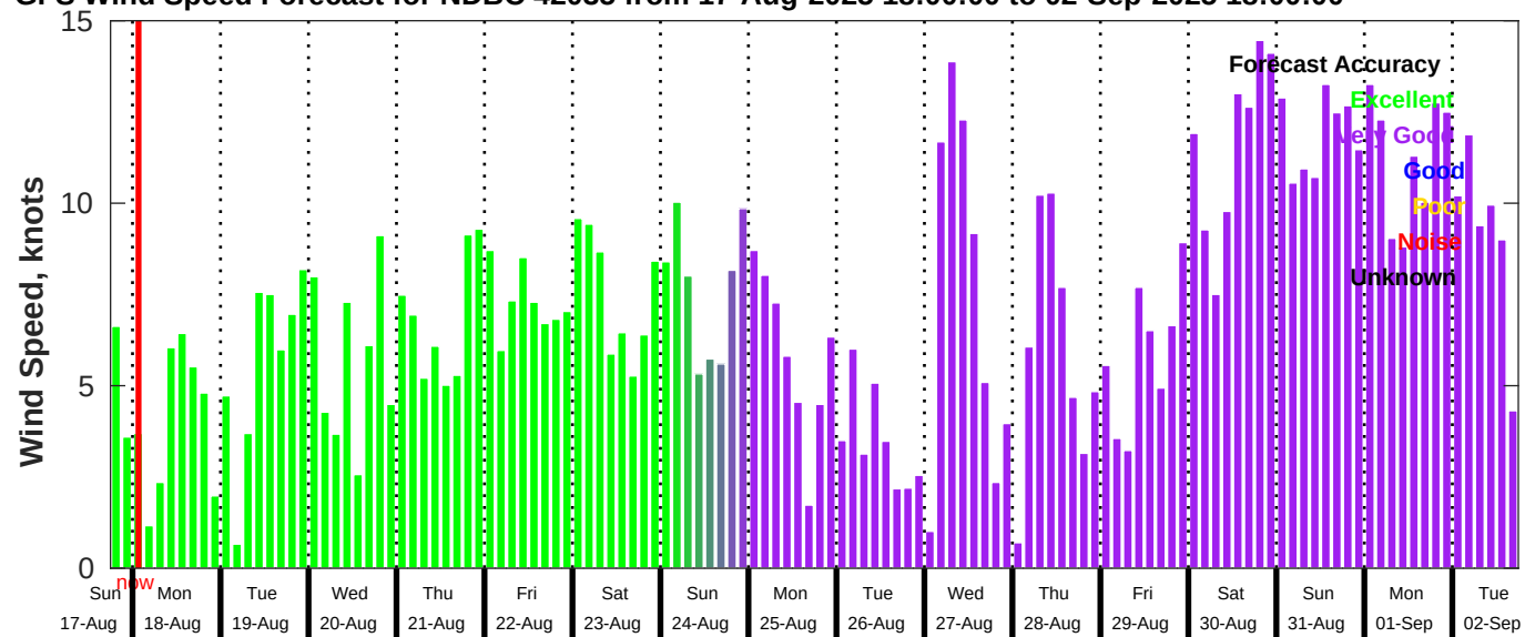
GFS Wind Speed Forecast for NDBC 42035 from 17-Aug-2025 18:00:00 to 02-Sep-2025 18:00:00
