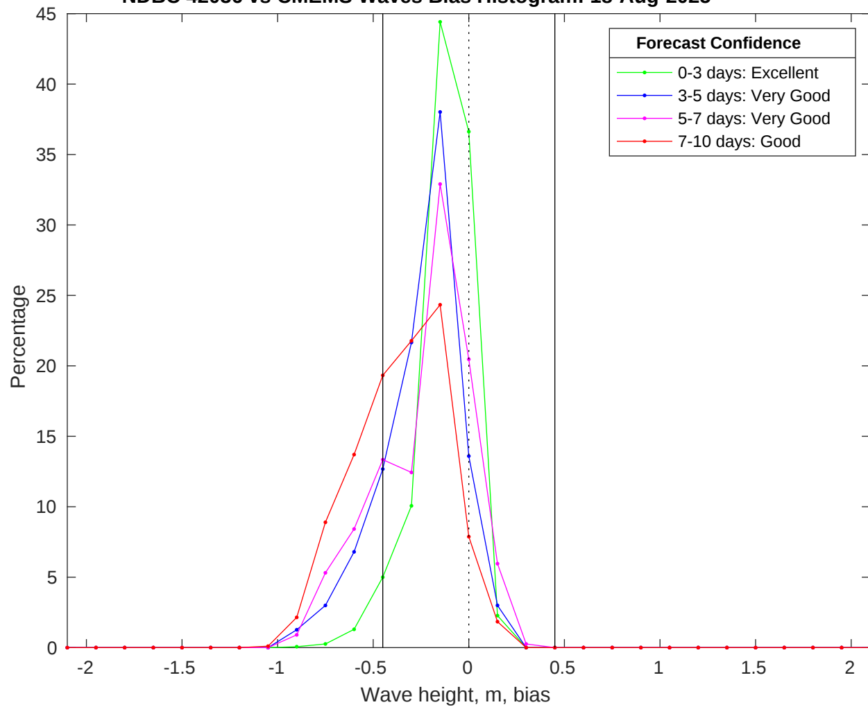
NDBC 42036 vs CMEMS Waves Bias Histogram: 18-Aug-2025
