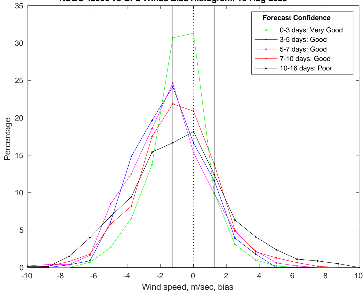
NDBC 42036 vs GFS Winds Bias Histogram: 18-Aug-2025
