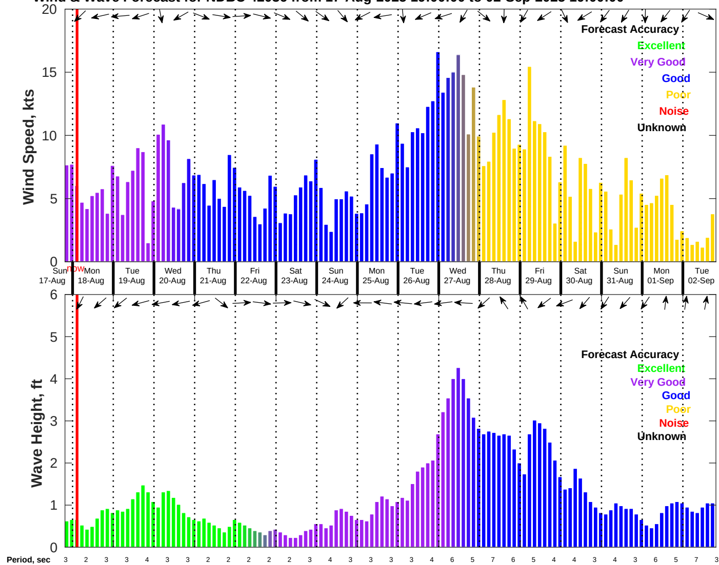
Wind & Wave Forecast for NDBC 42036 from 17-Aug-2025 19:00:00 to 02-Sep-2025 19:00:00
