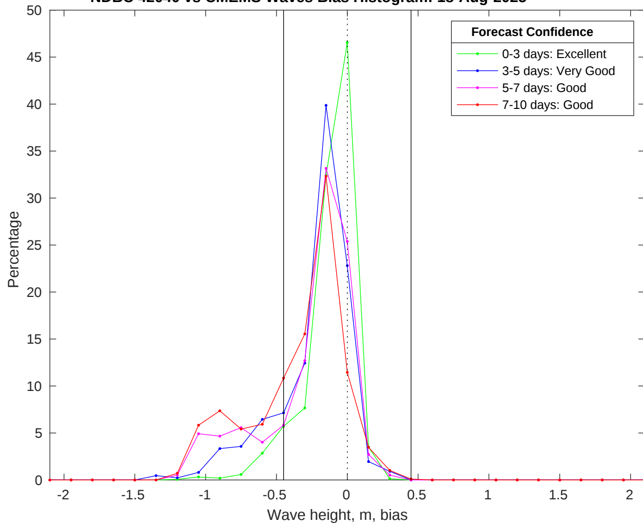
NDBC 42040 vs CMEMS Waves Bias Histogram: 18-Aug-2025
