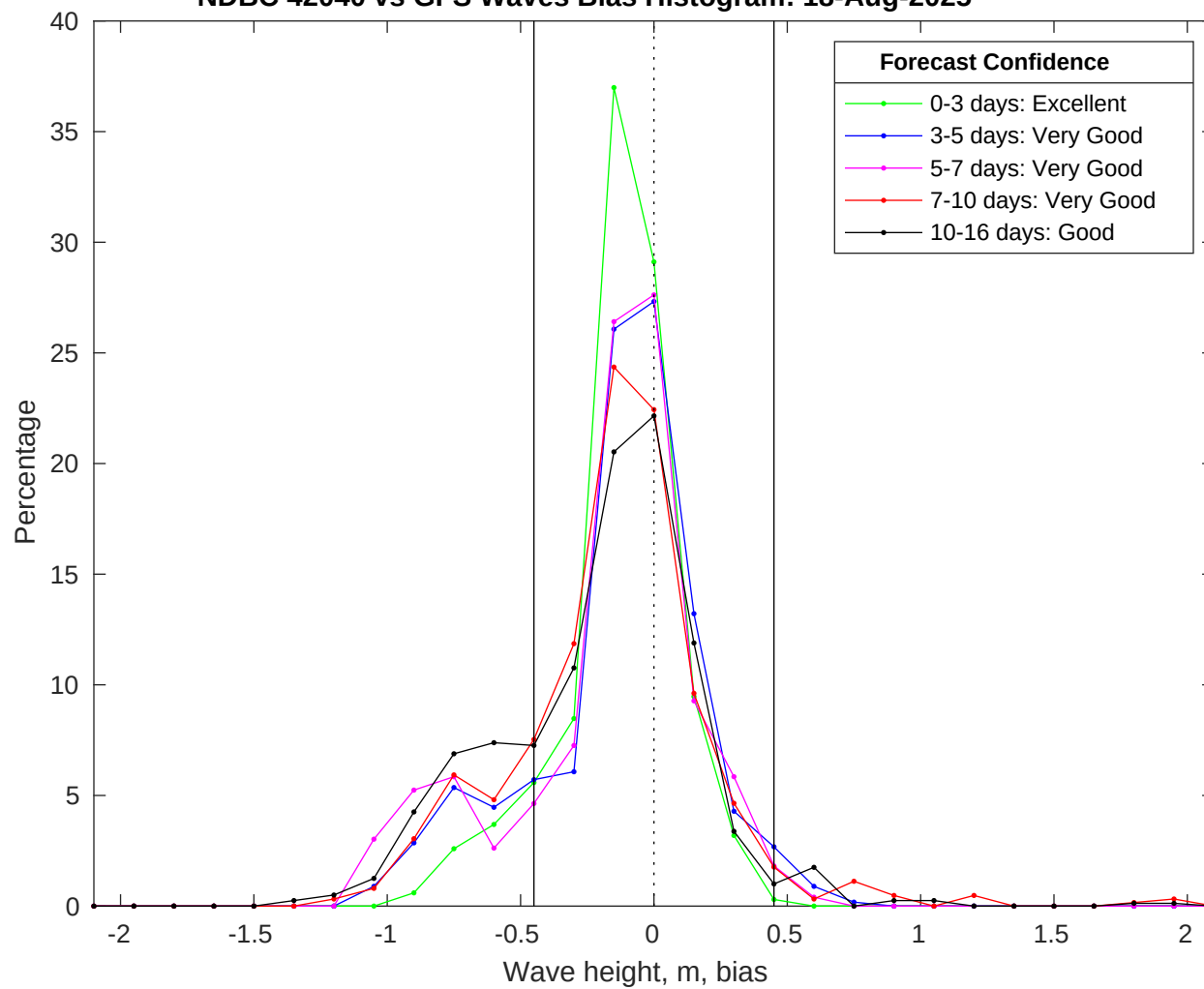
NDBC 42040 vs GFS Waves Bias Histogram: 18-Aug-2025
